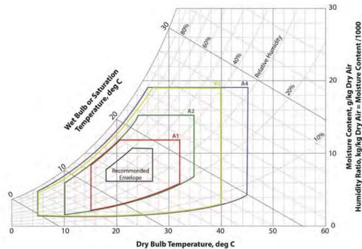
Figure 1. ASHRAE Temperature & Relative Humidity Recommendations for Data Centers
